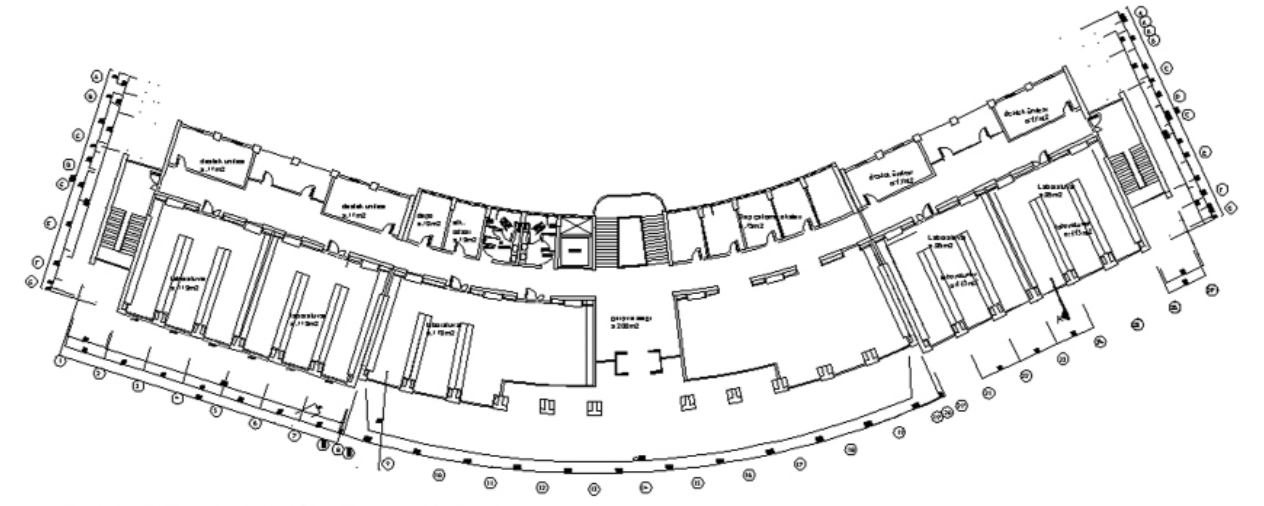
±0.00 KOTU ZEMİN KAT PLANI
